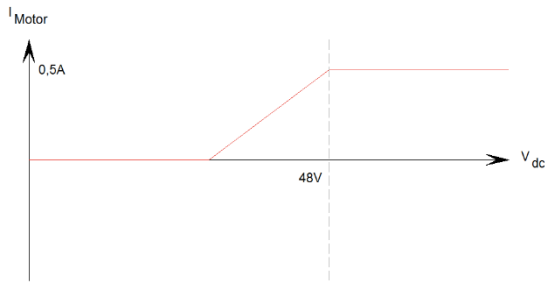
Figure 2: Droop control for a Dc motor
