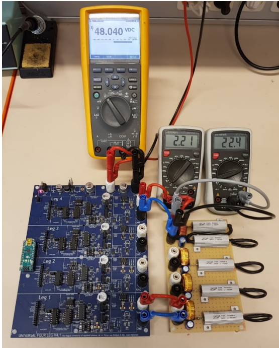
Figure 9: Laboratory setup with 4 passive loads.
