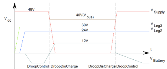
Figure 8: Droop control with Voltage drop, charge and discharge of a battery and overall stabilizing of the legs/outputs.
