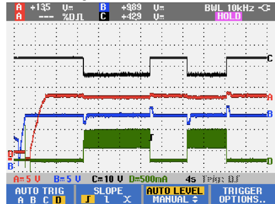
Figure 7: At 48V on the Input voltage of the U4L (Vbus), Input C, a stable pulse-width of respectively 15V & 10V on Leg one & two of the U4L at Input A & B of the scope. Input D shows the current going through Leg one/Input A.
