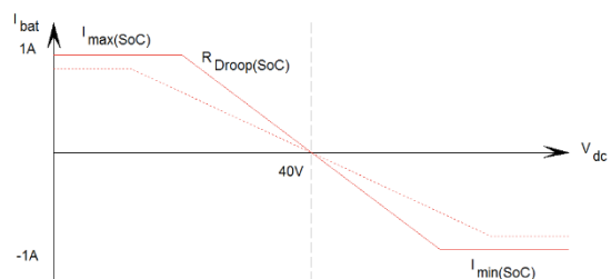
Figure 4: Droop control for a rechargeable battery
