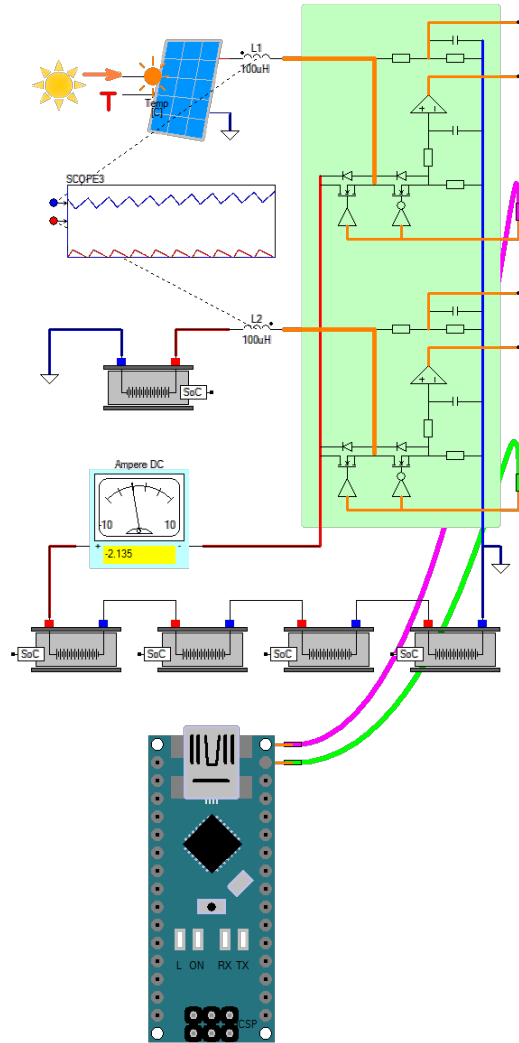
Figure 6: Simulation[3] of a grid manager with droop control and two legs. Leg 1 controls the solar panel using a build in maximum power point tracker, while leg 2 includes the droop characteristic for a rechargeable battery.
