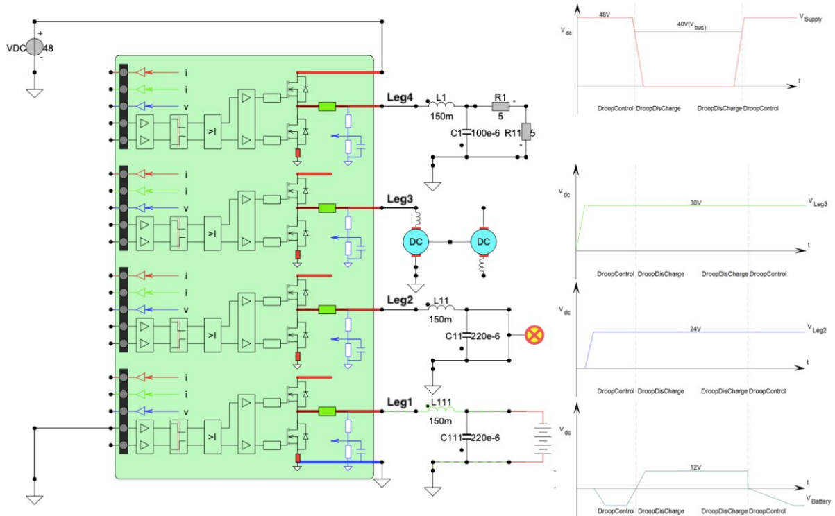
Figure 1: U4L configured as laboratory set up power from top to bottom; Passive load, Dc motor, light and a rechargeable battery.
