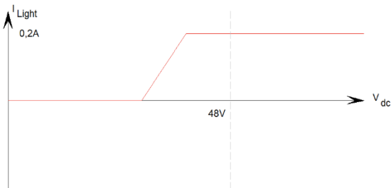
Figure 3: Droop control for lighting
